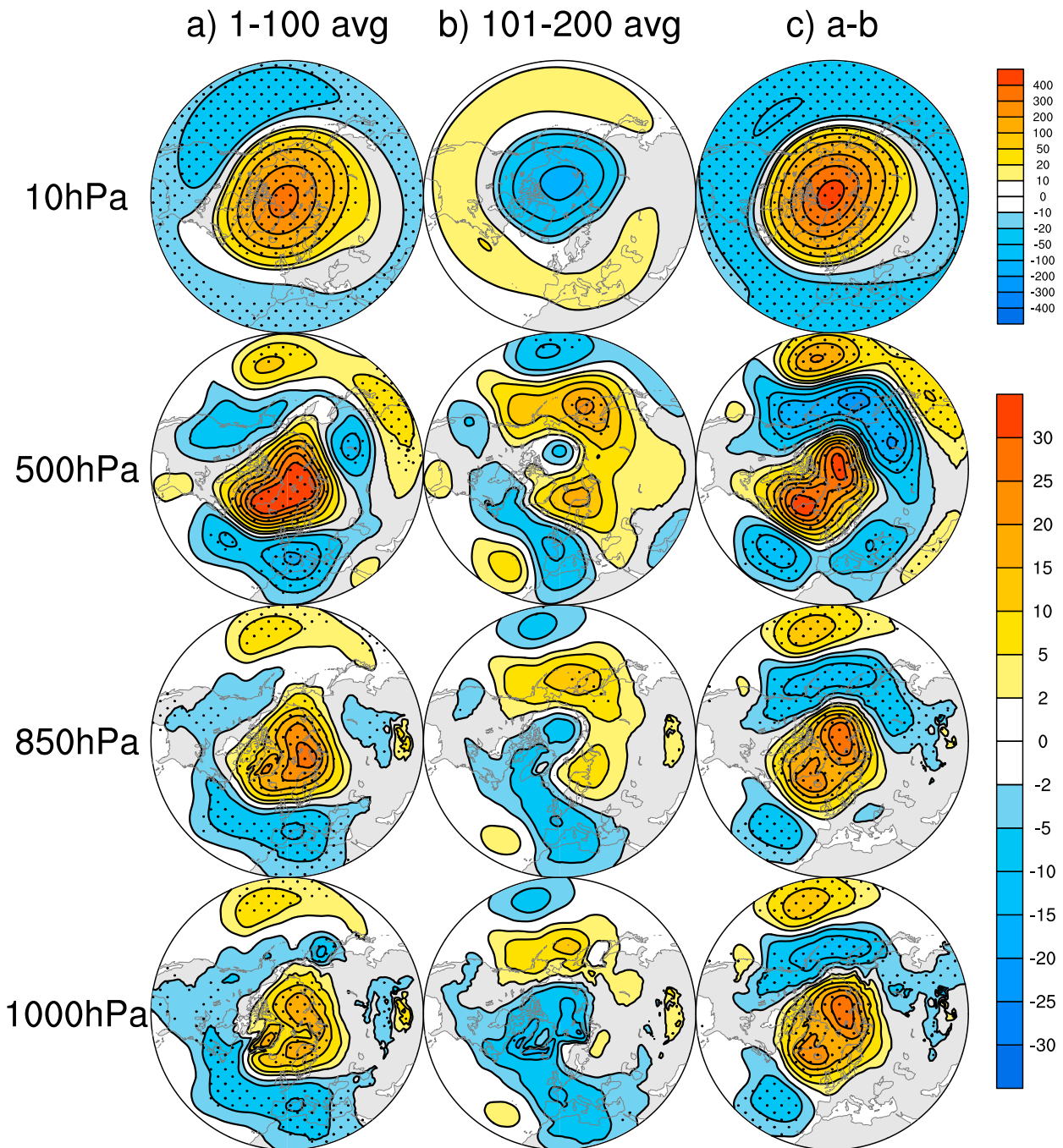
FIG. 6. Geopotential height response (m) in \Delta\text{past}_{\text{piST}} for the (a) first 100-member average and (b) second 100-member average, and (c) their difference. (from top to bottom) The 10-hPa DJF response and the 500-, 850- and 1000-hPa responses in JFM, respectively. Stippling indicates the 90% statistical significance based on a two-sided Student's t test and false discovery rate.
