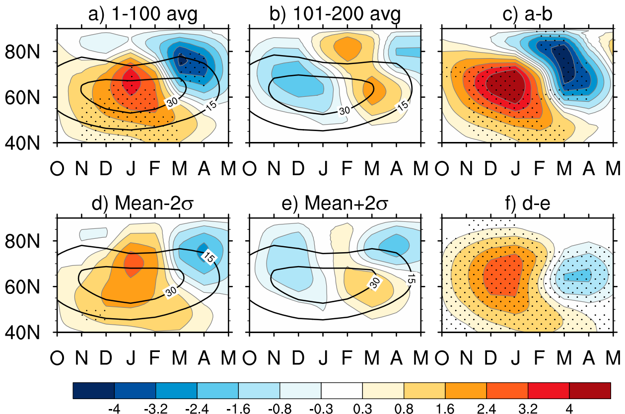
FIG. 11. (top) Eddy heat flux response near 100 hPa (model hybrid 0.1 sigma level; shading: \text{K m s}^{-1} ) in \Delta\text{past}_{\text{piSST}} as a function of month (x axis) and latitude (y axis) for the (a) first 100-member average and (b) second 100-member average, and (c) their difference. (bottom) Regression analysis of eddy heat flux response near 100 hPa onto U10 across the 1000 bootstrapped samples of 100-member averages: (d) Mean - 2\sigma , (e) Mean + 2\sigma , and (f) their difference. Stippling indicates the 90% statistical significance based on a two-sided Student's t test and false discovery rate. The climatologies (contours; interval of 15 \text{ K m s}^{-1} ) are overlaid on (a), (b), (d) and (e).
