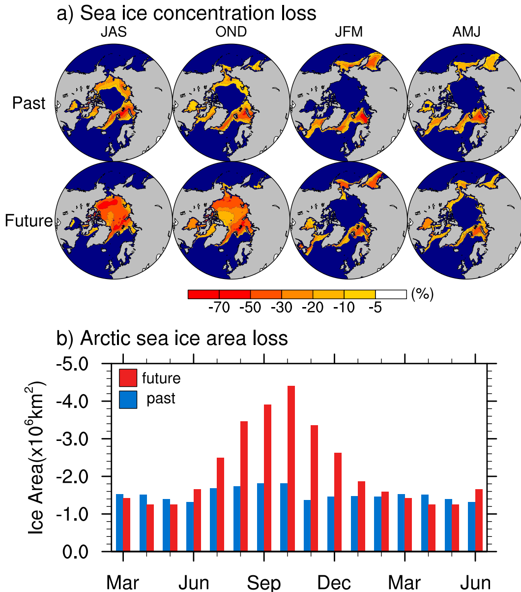
FIG. 1. (a) Seasonal maps of prescribed Arctic SIC loss (%) in the PAMIP experiments for the past (preindustrial to present day) and future (present day to +2^{\circ}\text{C} warming above preindustrial level). Summer, autumn, winter, and spring seasons are defined to be the average of July–September (JAS), October–December (OND), January–March (JFM), and April–June (AMJ), respectively. (b) Monthly Arctic sea ice area loss ( 10^6 \text{ km}^2 ) for the past (blue) and future (red); note the inverted y-axis scale.
