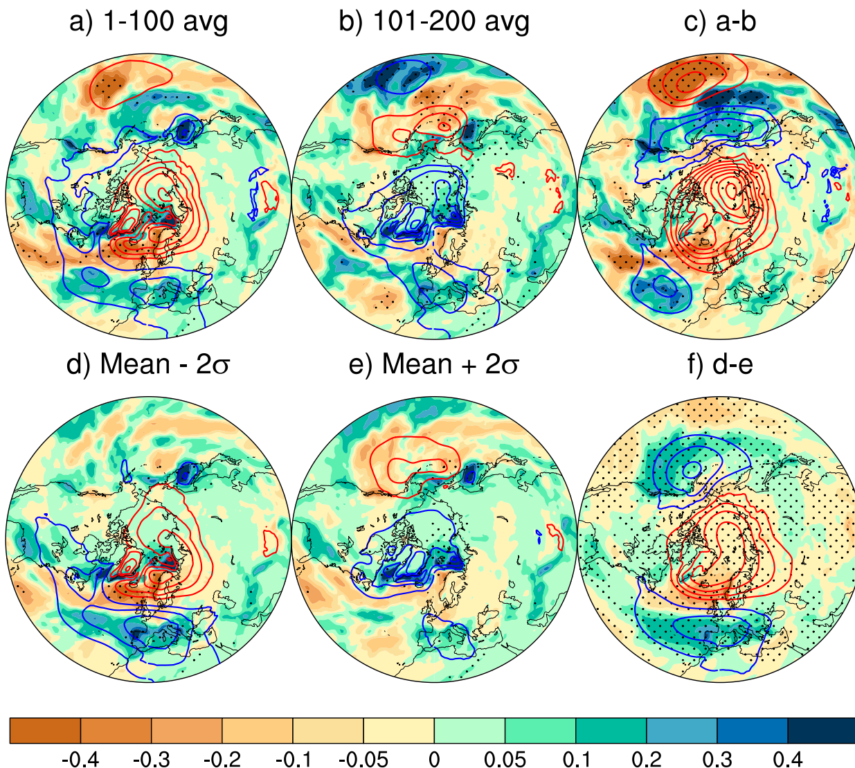
FIG. 9. (top) JFM precipitation (shading; \text{mm day}^{-1} ) and SLP (contours; interval of 0.5 hPa) responses in \Delta\text{past}_{\text{pisST}} for the (a) first 100-member average and (b) second 100-member average, and (c) their difference. (bottom) Regression analysis of JFM precipitation response onto U10 in \Delta\text{past}_{\text{pisST}} across the 1000 bootstrapped samples of 100-member averages: (d) Mean - 2\sigma , (e) Mean + 2\sigma , and (f) their difference. Red and blue contours denote positive and negative values, respectively. Zero contour line has been omitted. Stippling indicates the 90% statistical significance based on a two-sided Student's t test and false discovery rate.
