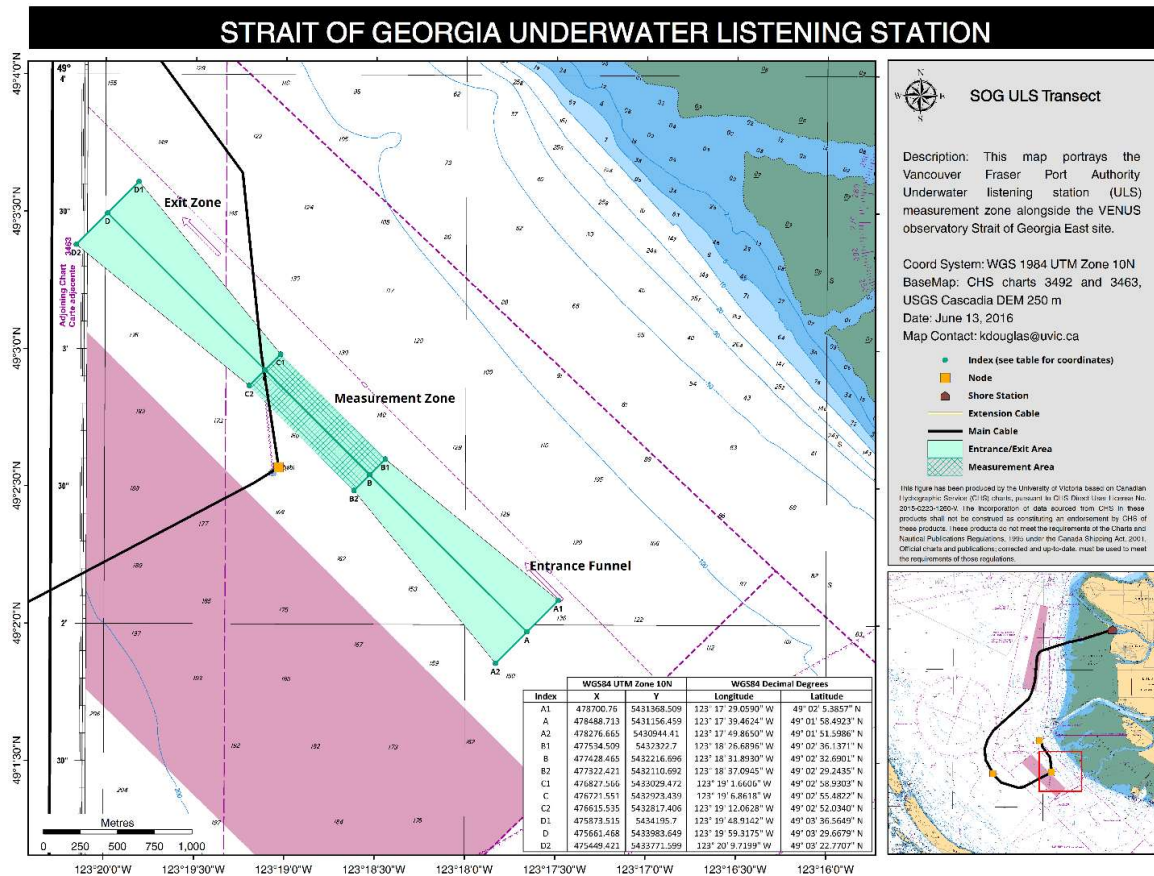
Figure B-3. Underwater Listening Station (ULS) location (yellow circle) at the VENUS East Node in Georgia Strait. Pilots use the measurement funnel (cyan) to ensure vessel source level measurements are accurate. Figure reproduced from MacGillivray et al. (2018).
