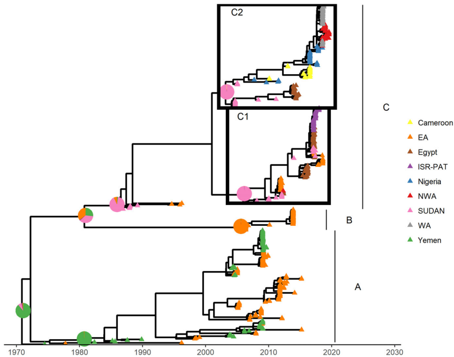
FIGURE 2 Maximum clade credibility trees of the O/EA-3 FMDV toptype. Colours represent the country or region where the sequences were collected for the tips (triangle) or where the node was predicted to be located (pie chart). The vertical lines (A–C) represent the clades identified and the boxes C1 and C2, the two subclades of clade C
