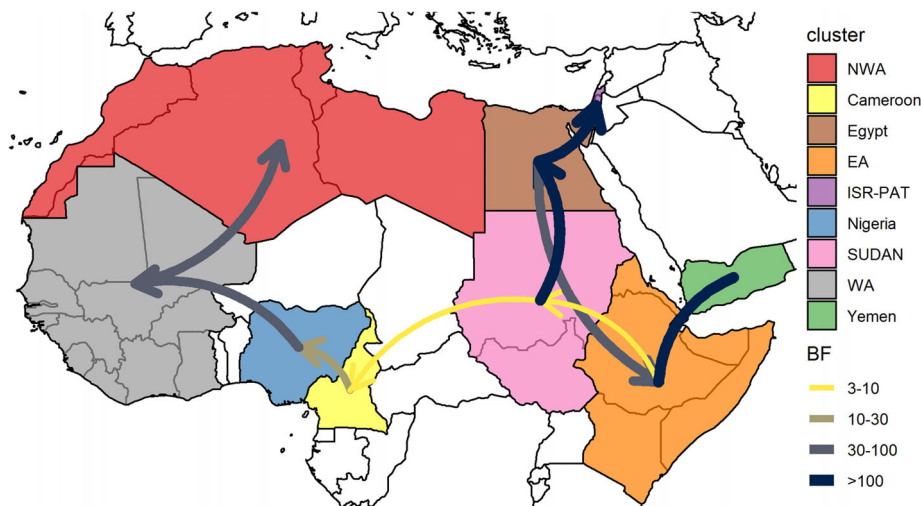
FIGURE 3 Migration routes predicted for the O/EA-3 FMDV toptype by the discrete state phylogeography analysis. Filled geographical areas represent the countries or regions. The arrows represent the supported migrations. The level of support (Bayes factor, BF) is represented by the arrows' colours and thickness: moderate support for 3 \leq BF < 10 , strong support for 10 \leq BF < 30 , very strong support for 30 \leq BF < 100 and extreme support for BF \geq 100
