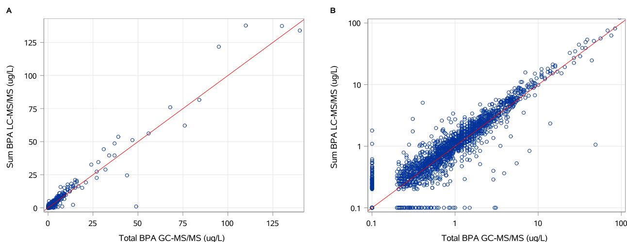
Fig. 1. Scatterplot of Total BPA (indirect GC-MS/MS) (µg/L) and Sum BPA (direct LC-MS/MS) (µg BPA equivalents/L) with identity diagonal in red (panel A), and with a log-10 scale for both axes (panel B). LOD = 0.2 µg/L, LOD/2 imputation. (For interpretation of the references to colour in this figure legend, the reader is referred to the web version of this article.)
