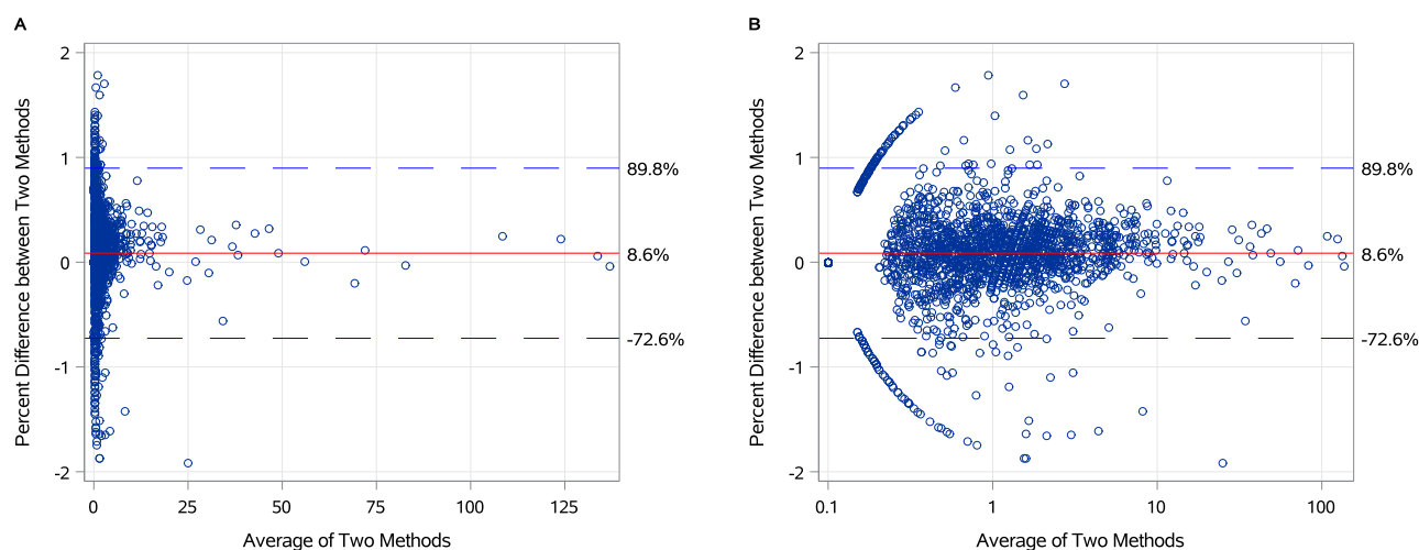
Fig. 2. Bland-Altman analysis of percentage differences (panel A), and x-axis in log-10 scale (panel B). LOD = 0.2 µg/L, LOD/2 imputation.
