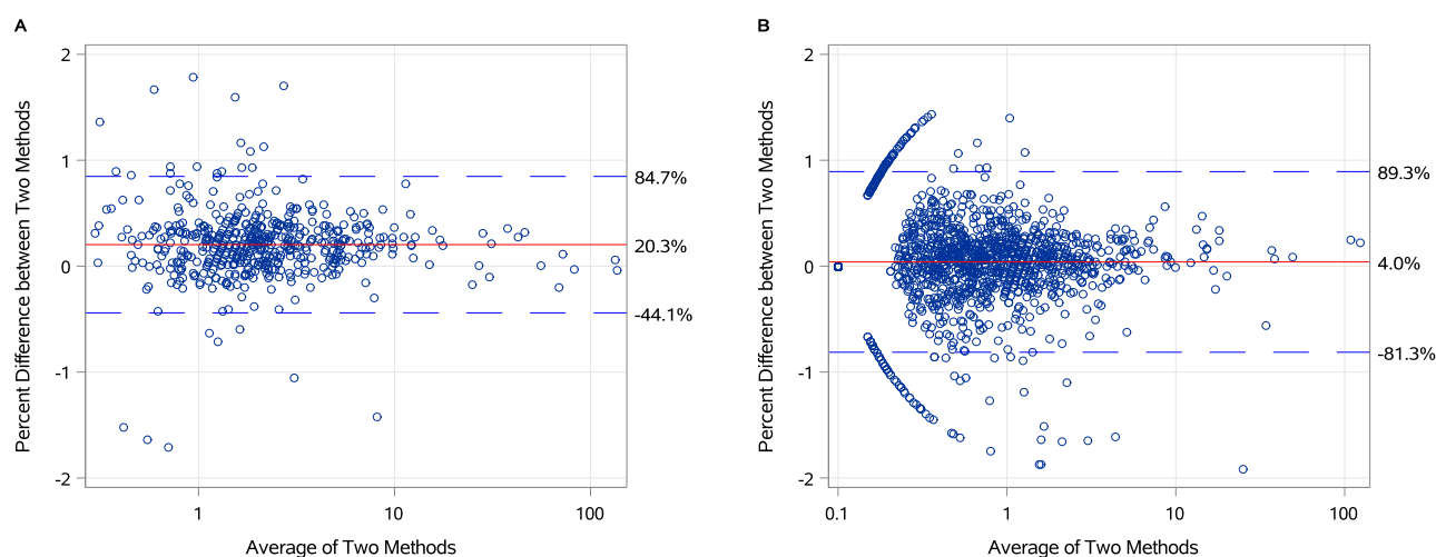
Fig. 3. Bland-Altman analysis of percentage differences stratified according to urinary specific gravity ≥ 1.02 (panel A) and < 1.02 (panel B) with x axis in log-10 scale.
