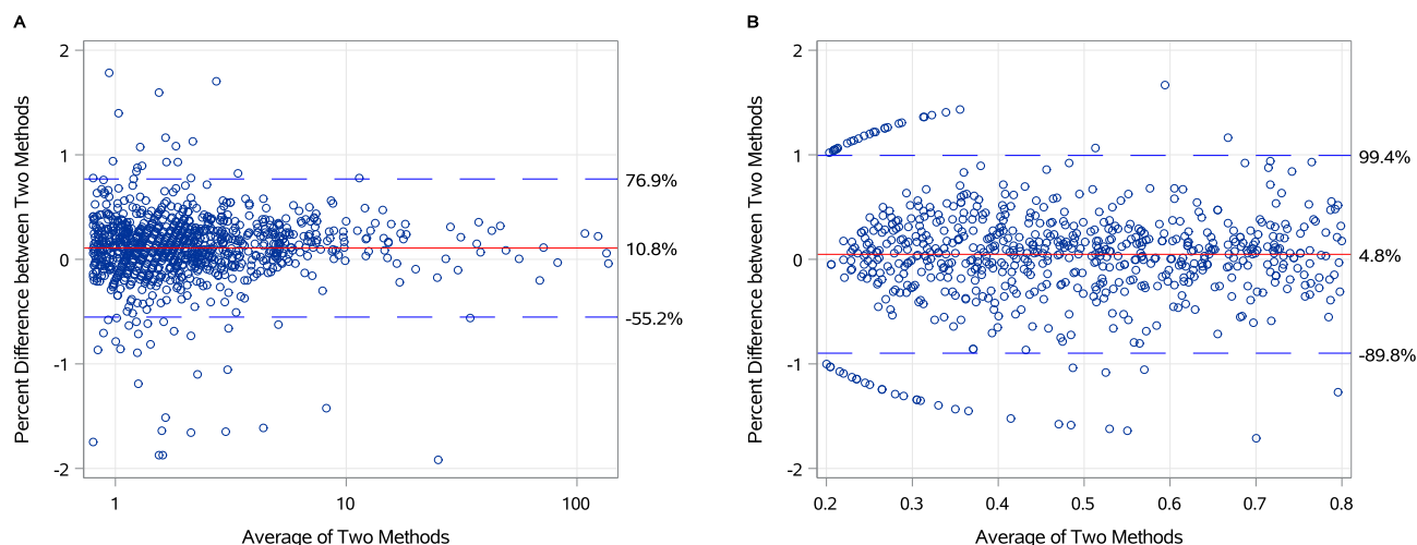
Fig. 4. Bland-Altman analysis of percentage differences stratified according to values equal to or above LOQ ( \geq 0.8 \mu\text{g/mL} ) with x-axis in log-10 scale (panel A) and values between the LOD and LOQ (panel B) ( 0.2 - < 0.8 \mu\text{g/mL} ).
